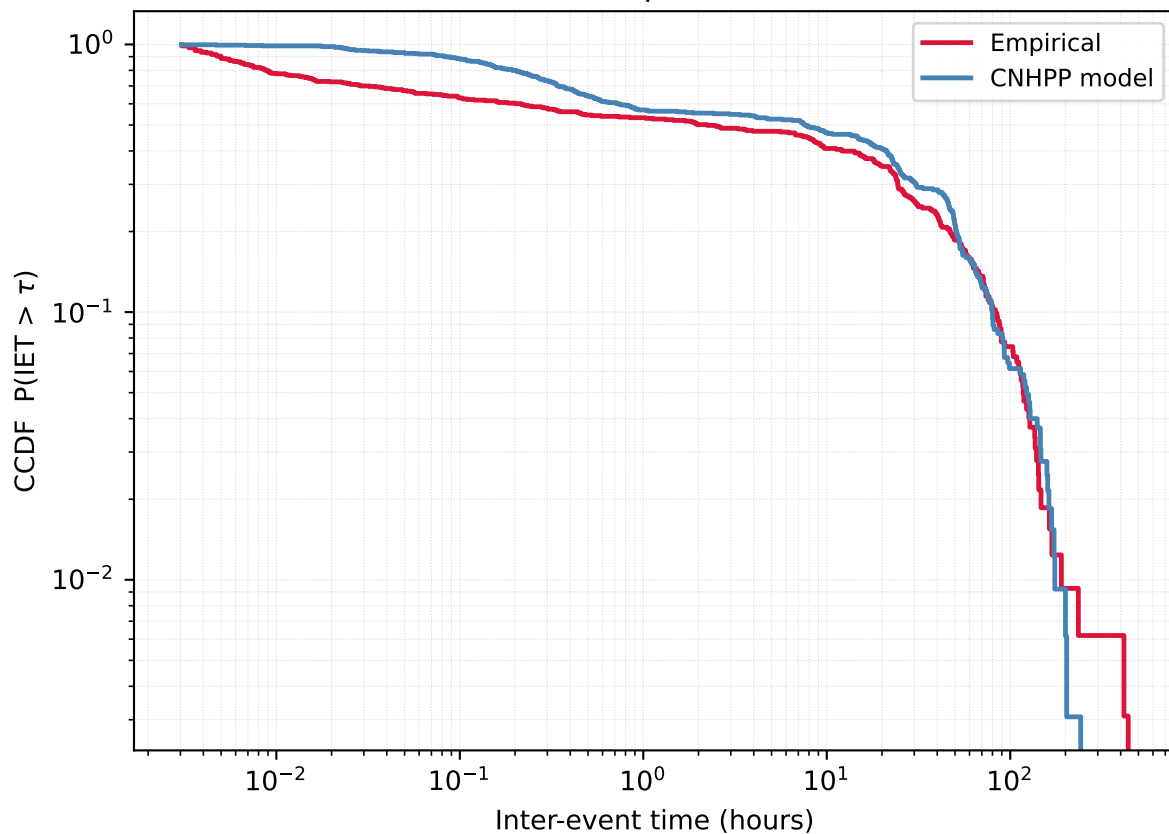
User 302926911 - Empirical vs CNHPP model
