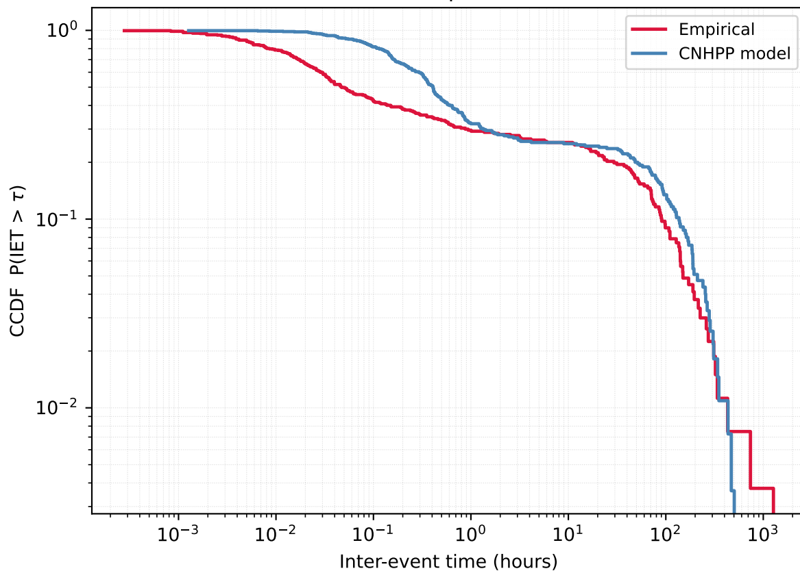
User 1848901170 - Empirical vs CNHPP model
