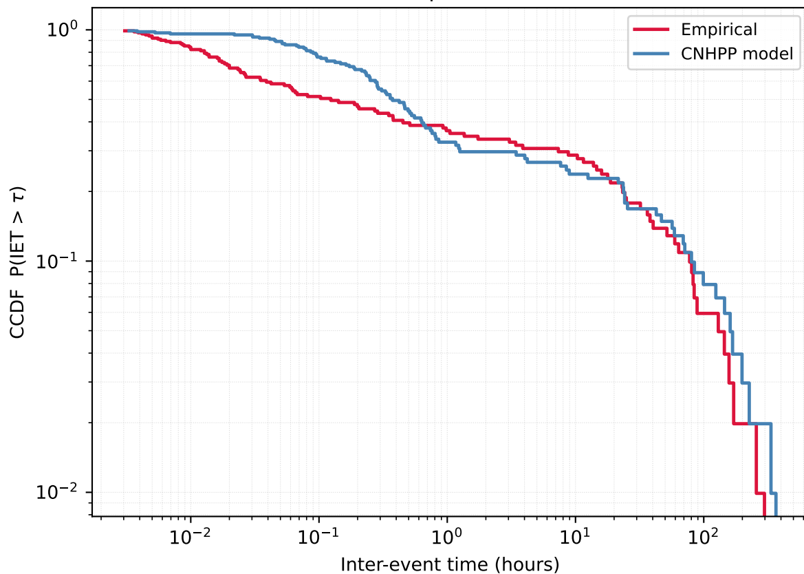
User 5357949 - Empirical vs CNHPP model
