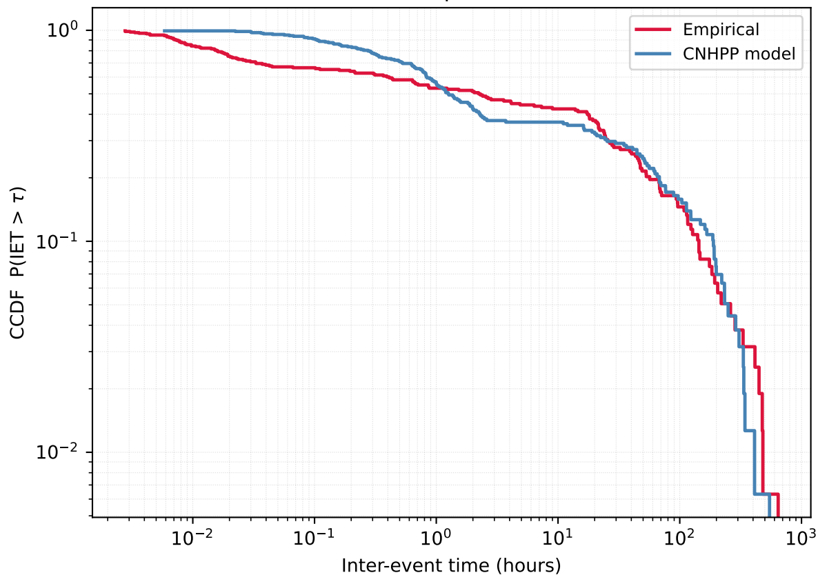
User 170506767 - Empirical vs CNHPP model
