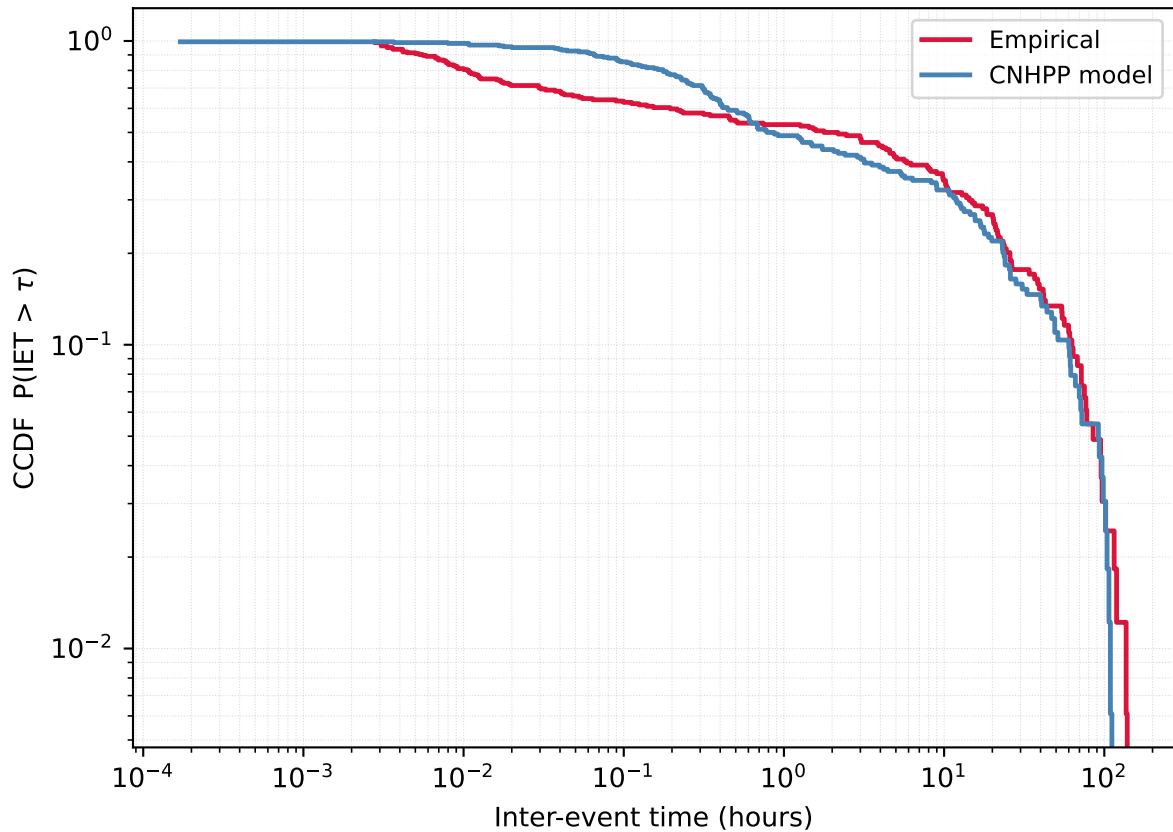
User 34343445 - Empirical vs CNHPP model
