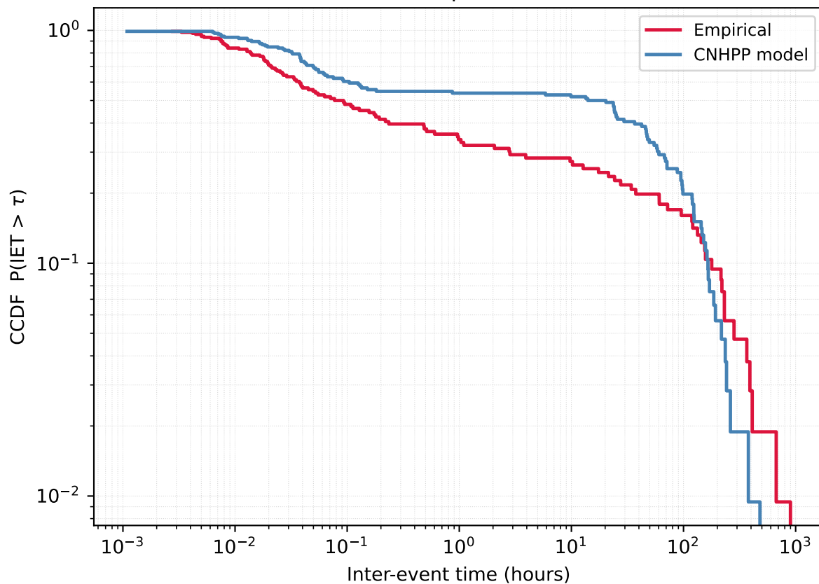
User 185880661 - Empirical vs CNHPP model
