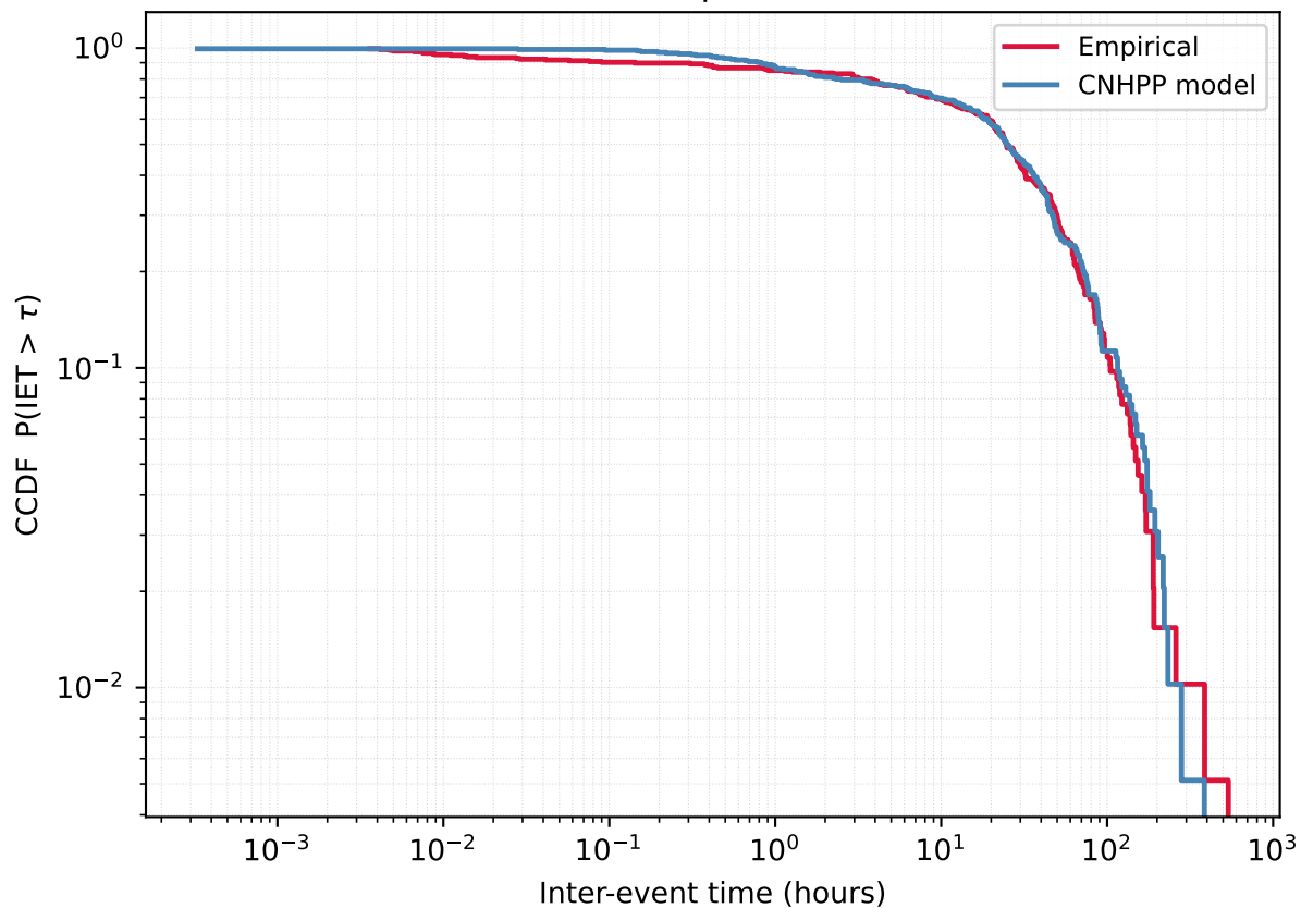
User 428716184 - Empirical vs CNHPP model
