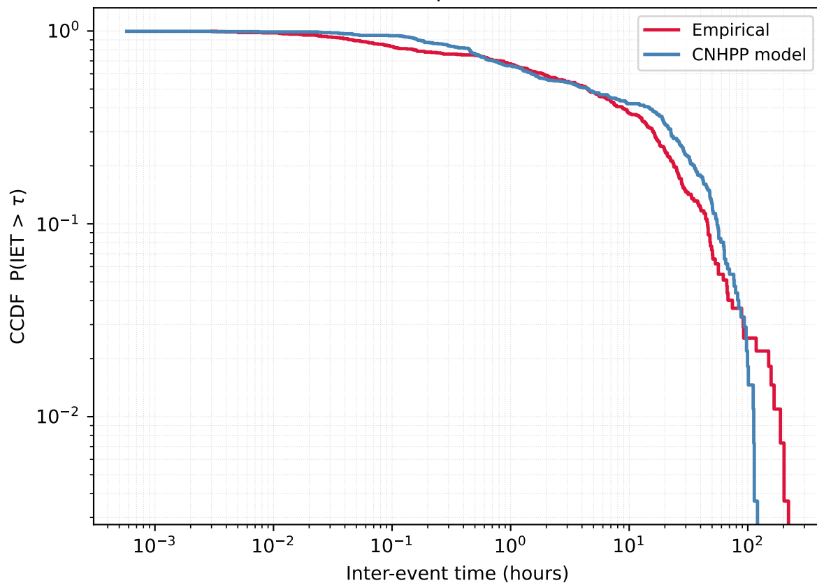
User 1232695 - Empirical vs CNHPP model
