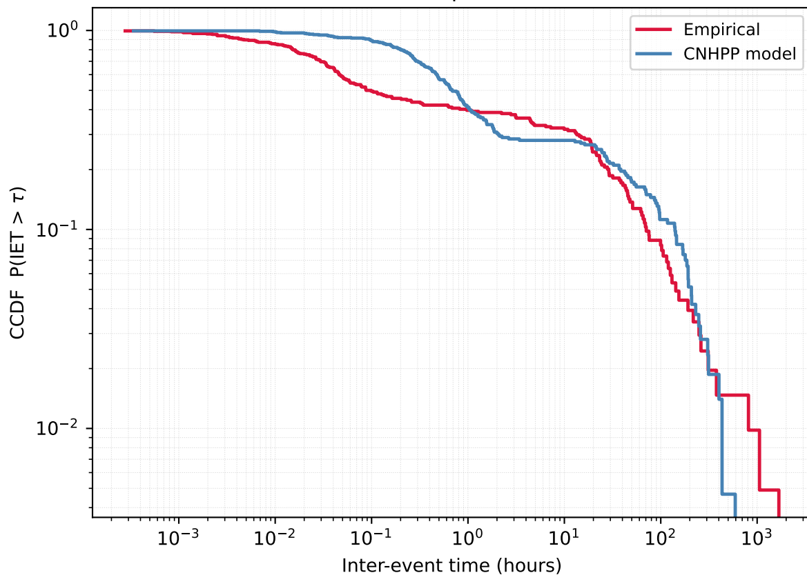
User 1366797899 - Empirical vs CNHPP model
