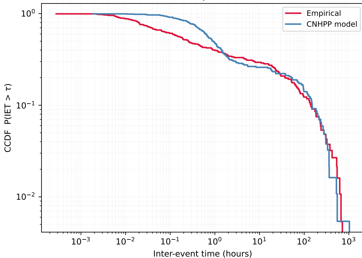
User 1992063859 - Empirical vs CNHPP model
