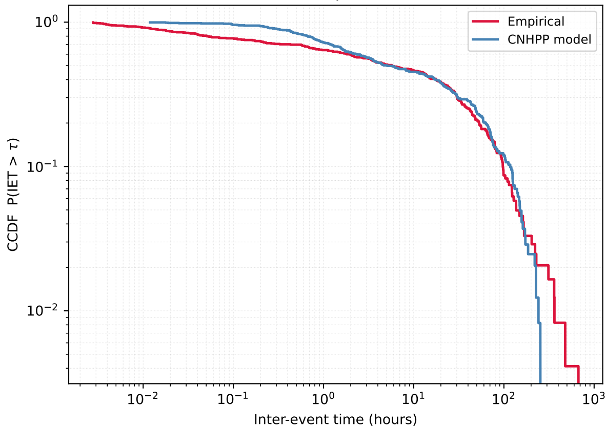
User 5561907303 - Empirical vs CNHPP model
