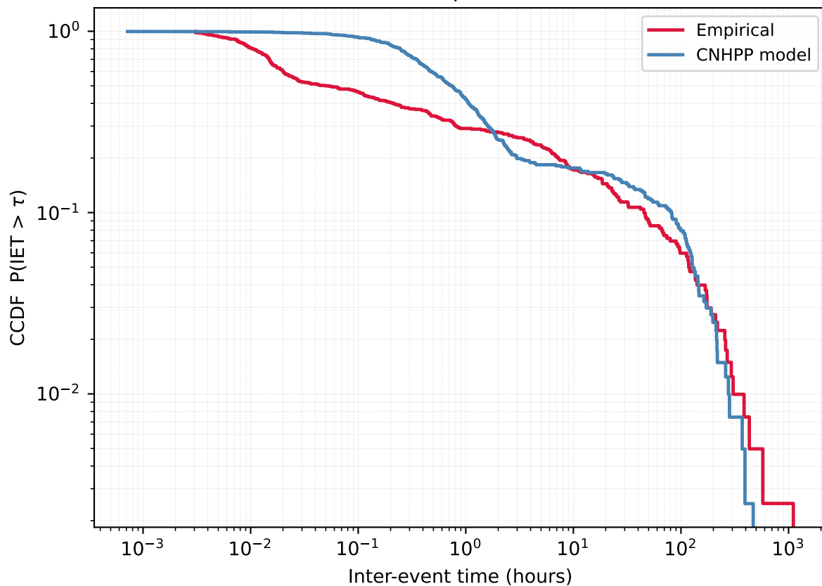
User 824741313 - Empirical vs CNHPP model
