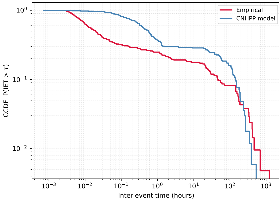
User 1843524645 - Empirical vs CNHPP model
