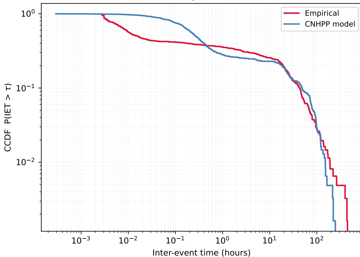
User 4473225 - Empirical vs CNHPP model
