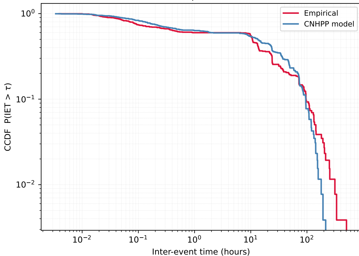
User 8786749 - Empirical vs CNHPP model
