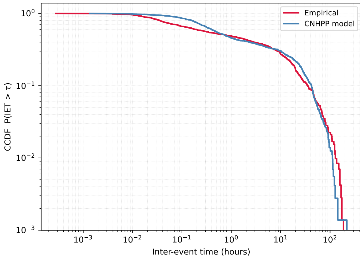
User 6988965722 - Empirical vs CNHPP model
