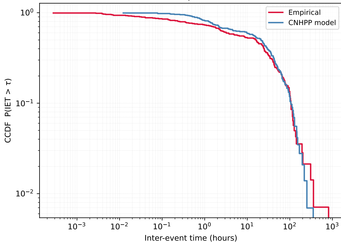
User 459294324 - Empirical vs CNHPP model
