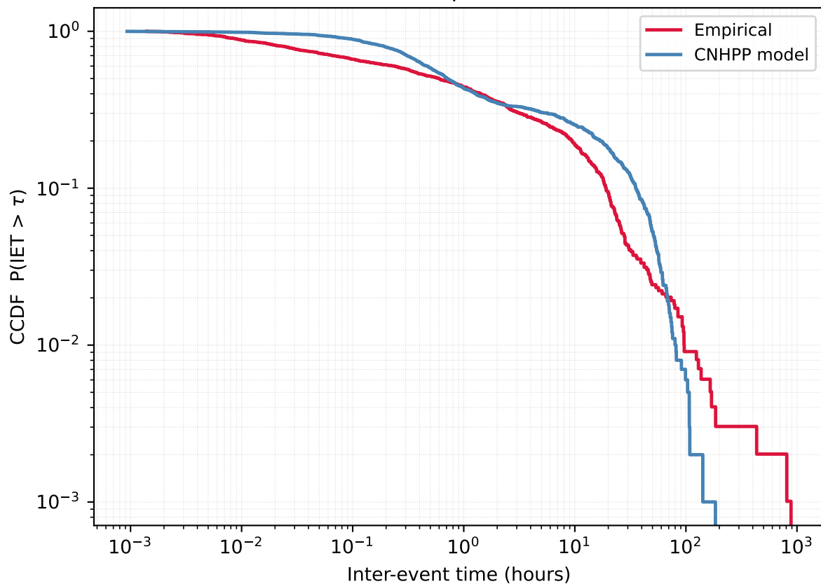
User 274636082 - Empirical vs CNHPP model
