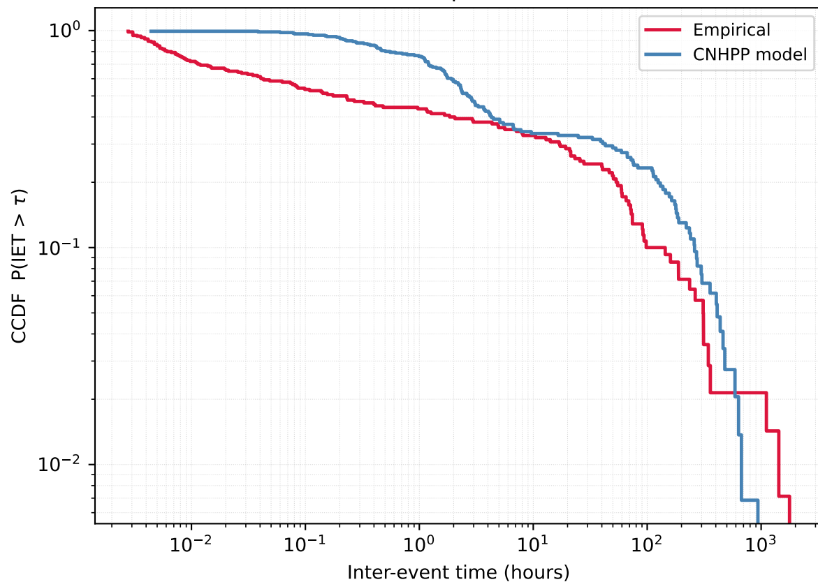
User 323309626 - Empirical vs CNHPP model
