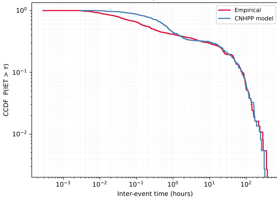
User 412633448 - Empirical vs CNHPP model
