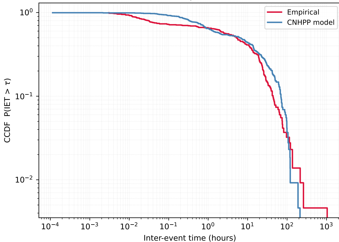
User 5657126860 - Empirical vs CNHPP model
