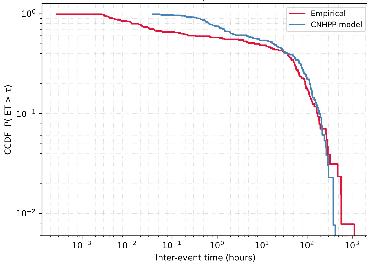
User 955992174 - Empirical vs CNHPP model
