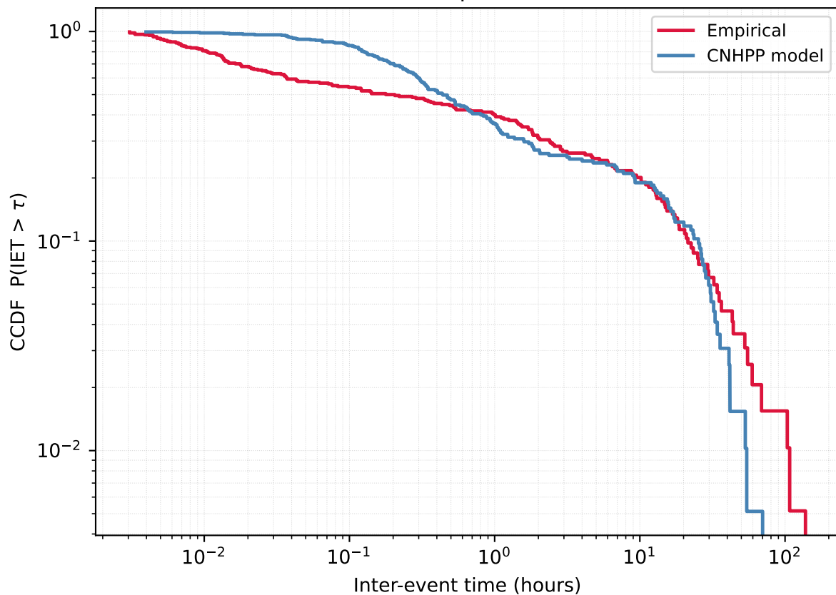
User 940028943 - Empirical vs CNHPP model
