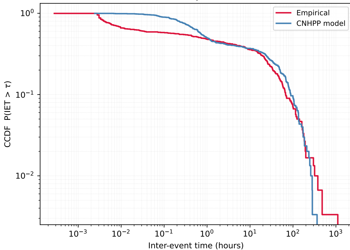
User 1273291262 - Empirical vs CNHPP model
